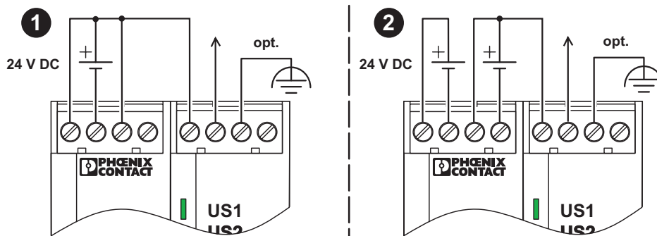
Figure 2 Example voltage supply of the module from one or two voltage sources and connection of the alarm contact
